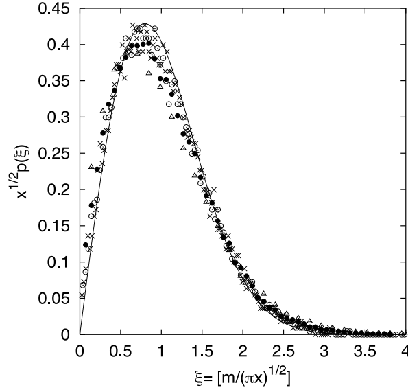
Figure 6. Numerical Monte Carlo scaling plot of the stationary state distribution p(m, x) , the probability to find a particle of mass m at site x , for various x = 16(\times) , 64(o) , 256(\bullet) , and 512(\Delta) . We plot \sqrt{x}p(x, m) versus \xi = m/\sqrt{\pi x} , the Gaussian form of equation (10).
