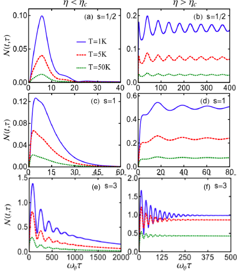
FIG. 2. The measure of non-Markovian dynamics in terms of two-time correlation function [29] for a bosonic system coupled to a thermal reservoir with Ohmic-type spectral density J(\epsilon) = 2\pi\eta\epsilon(\epsilon/\epsilon_c)^{s-1}e^{-\epsilon/\epsilon_c} . The energy cut-off \epsilon_c = 5\epsilon_s and the system is initially in Fock state with n = 1 , and t = 0 . As it is shown that when the system-reservoir coupling \eta < \eta_c , no localized bound state exists. Correspondingly, the transient two-time correlation function shows quantitatively that memory effect vanishes when the system approaches to the thermal equilibrium state; while in the strong coupling regime \eta > \eta_c , the existence of the localized bound state prohibits the system to approach to the equilibrium state, and the non-Markovian dynamics (memory effect) can remains forever.
