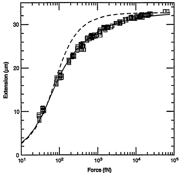
Fig. 1. Squares are experimental force versus extension data for 97 kb \lambda -DNA dimers from figure 3 of (2); solid line is a fit of the entropic force required to extend a worm-like polymer. The fit parameters are the DNA length ( L = 32.80 \pm 0.10 \mu\text{m} ) and the persistence length ( A = 53.4 \pm 2.3 \text{ nm} ). Shown for comparison (dashed curve) is the freely jointed chain model (2) with L = 32.7 \mu\text{m} and a segment length b = 100 \text{ nm} chosen to fit the small- x data.
