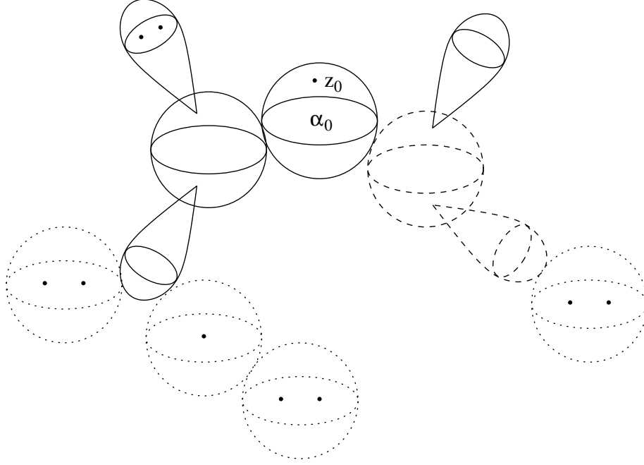
FIGURE 1. Stable map consisting of vortex classes over \mathbb{C} and pseudo-holomorphic spheres in \bar{M} .
